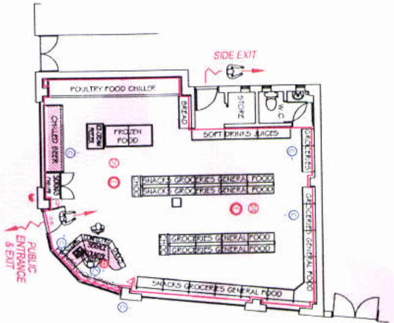
GROUND FLOOR PLAN LAYOUT
